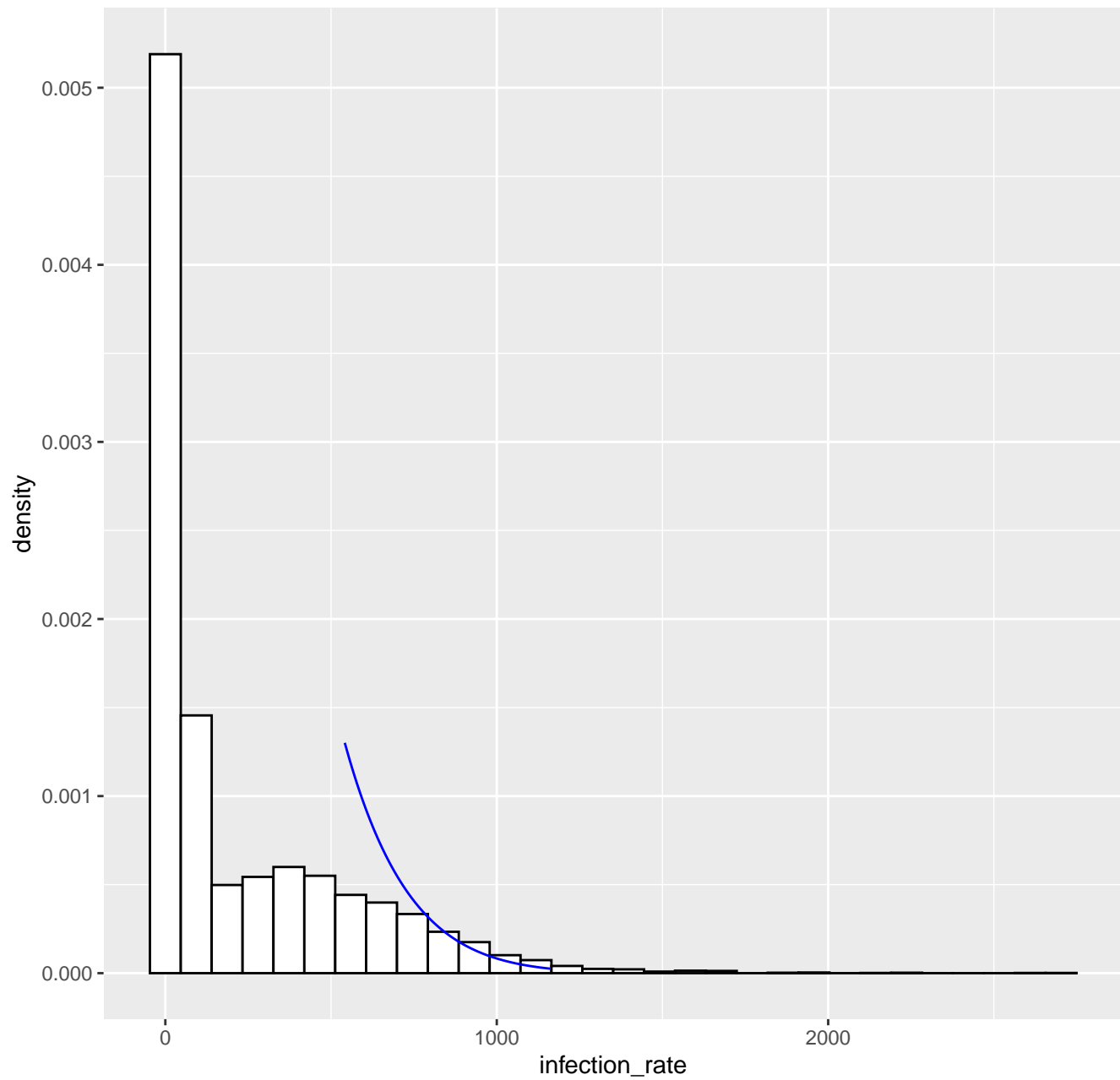
Fitted tail density GPD( 541.5 , 173.25 , -0.09 ), k= 80 -- 26-01-2021
