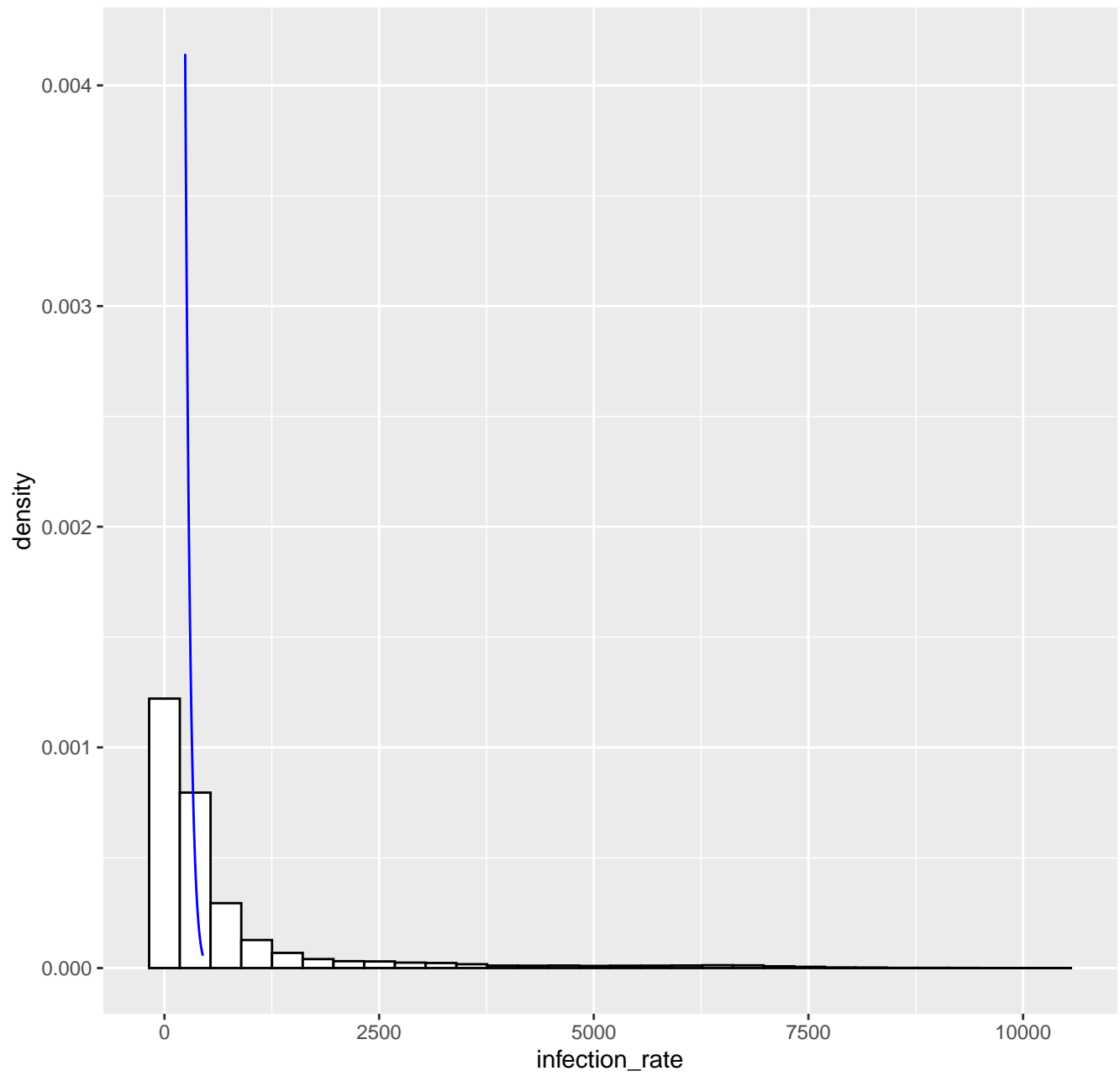
Fitted tail density GPD( 241.2 , 54.4 , -0.1 ), k= 80 -- 25-10-2022
