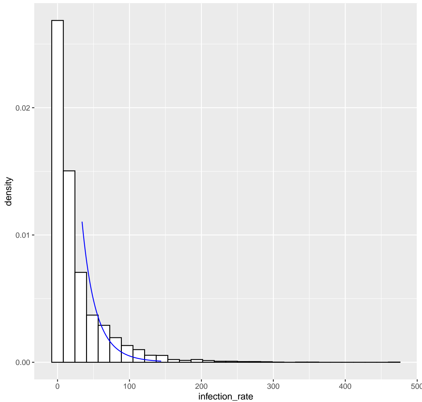
Fitted tail density GPD( 34.1 , 20.4 , 0.08 ), k= 80 -- 25-08-2020
