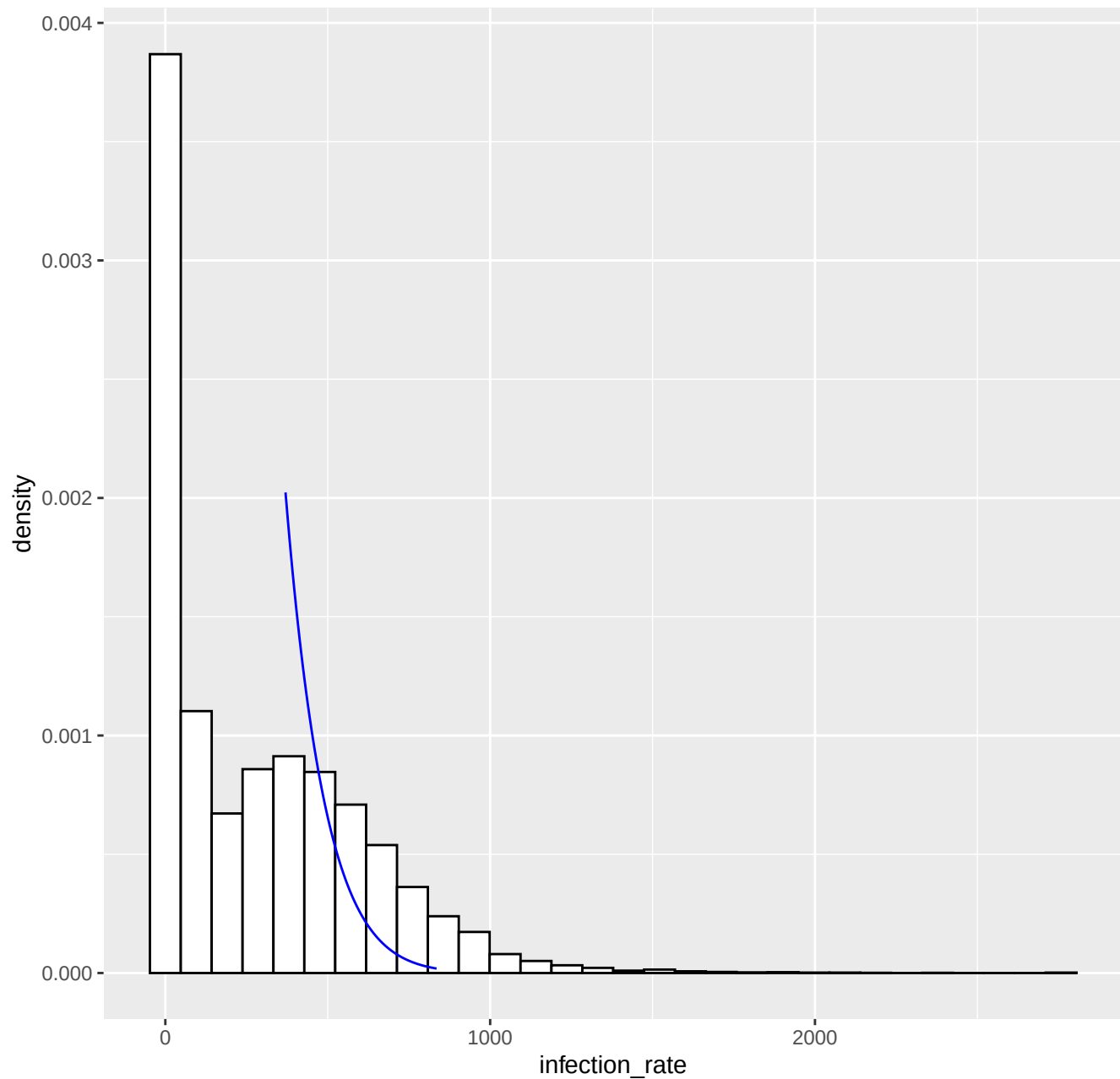
Fitted tail density GPD( 370 , 111.38 , -0.08 ), k= 80 -- 25-05-2021
