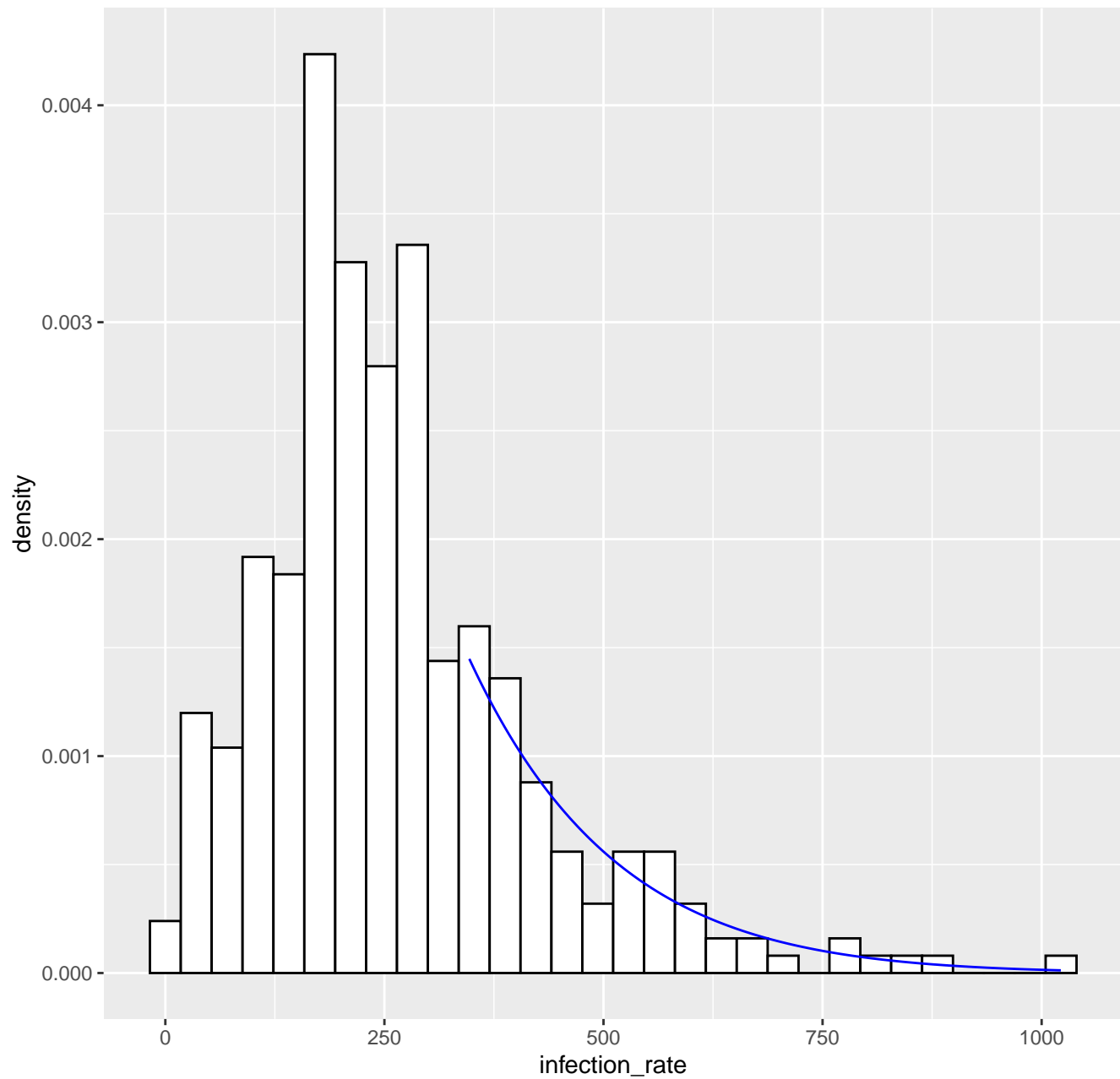
Fitted tail density GPD( 346.9 , 155.63 , -0.06 ), k= 80 -- 25-05-2020
