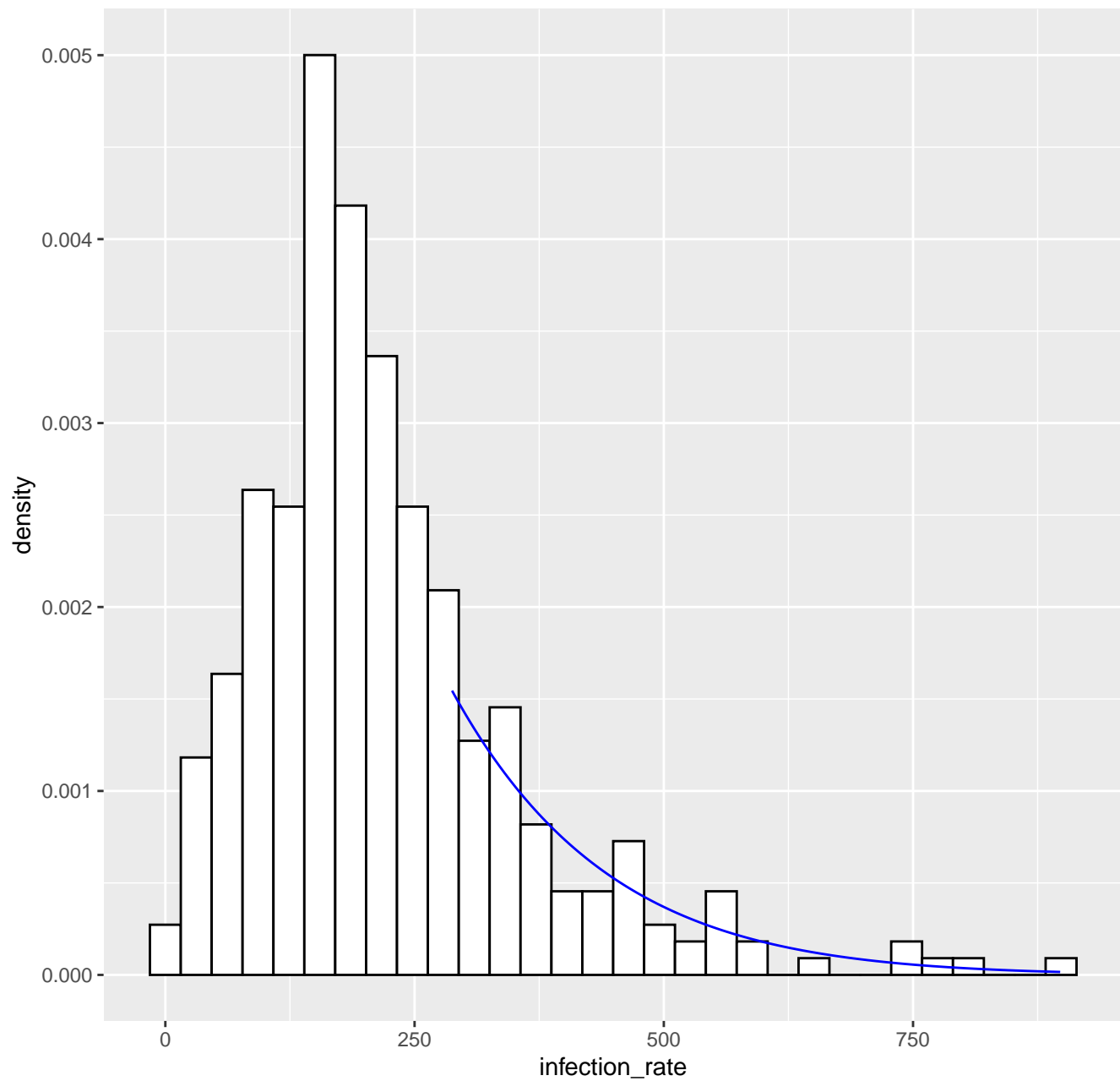
Fitted tail density GPD( 287.6 , 145.84 , -0.06 ), k= 80 -- 25-04-2020
