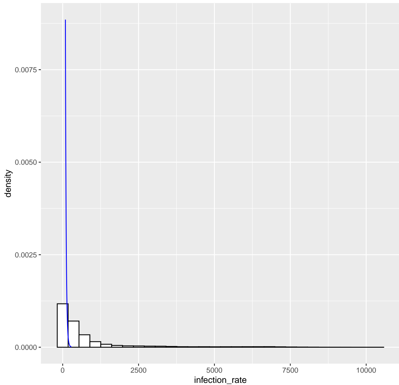
Fitted tail density GPD( 89.9 , 25.46 , 0.04 ), k= 80 -- 24-05-2022
