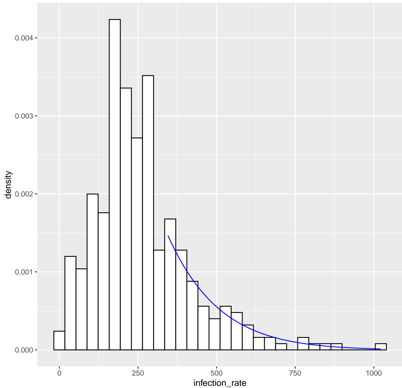
Fitted tail density GPD( 345.3 , 153.76 , -0.06 ), k= 80 -- 24-05-2020
