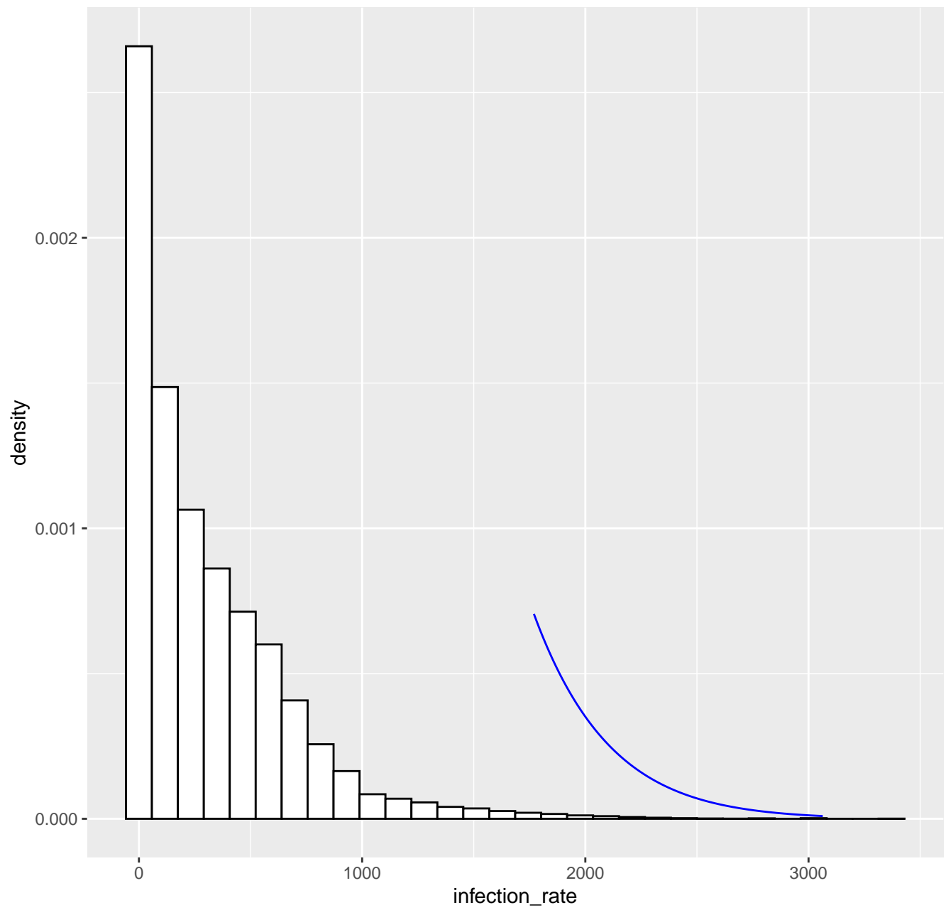
Fitted tail density GPD( 1769.6 , 319.5 , -0.05 ), k= 80 -- 23-11-2021
