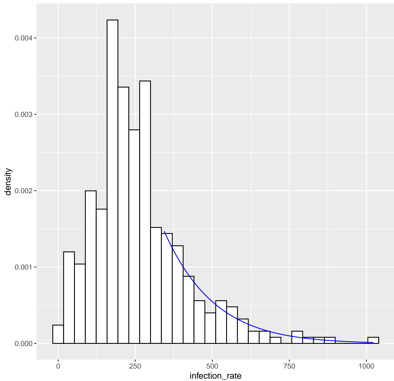
Fitted tail density GPD( 344.1 , 153.53 , -0.05 ), k= 80 -- 23-05-2020
