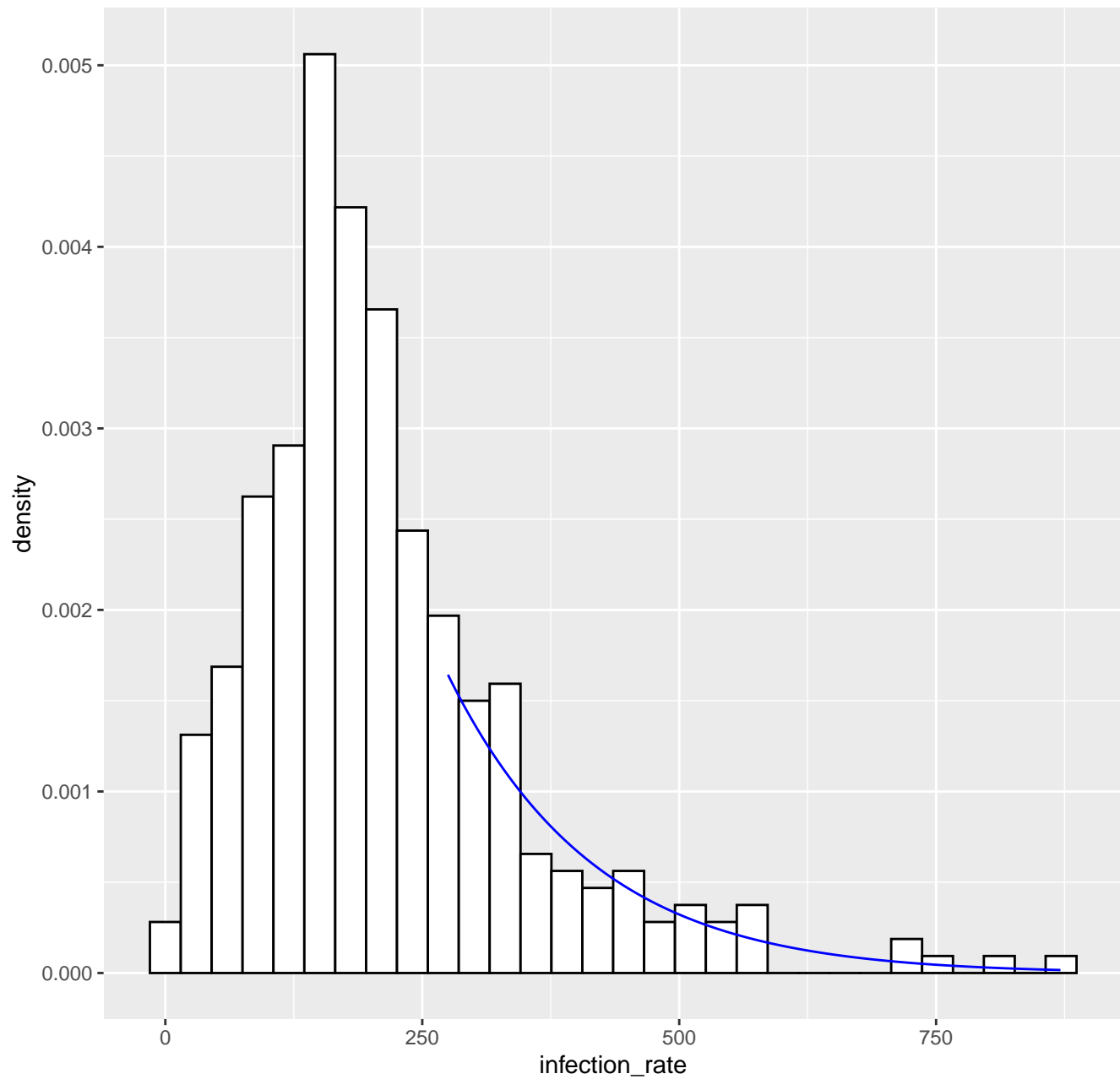
Fitted tail density GPD( 275 , 137.17 , -0.04 ), k= 80 -- 23-04-2020
