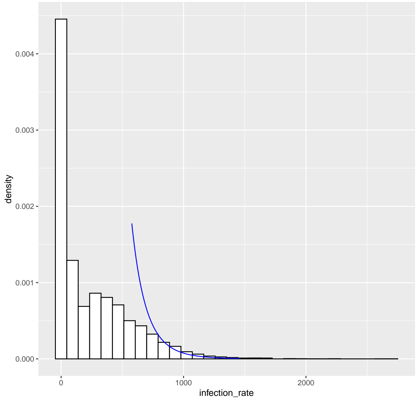
Fitted tail density GPD( 577.5 , 126.94 , 0.1 ), k= 80 -- 23-03-2021
