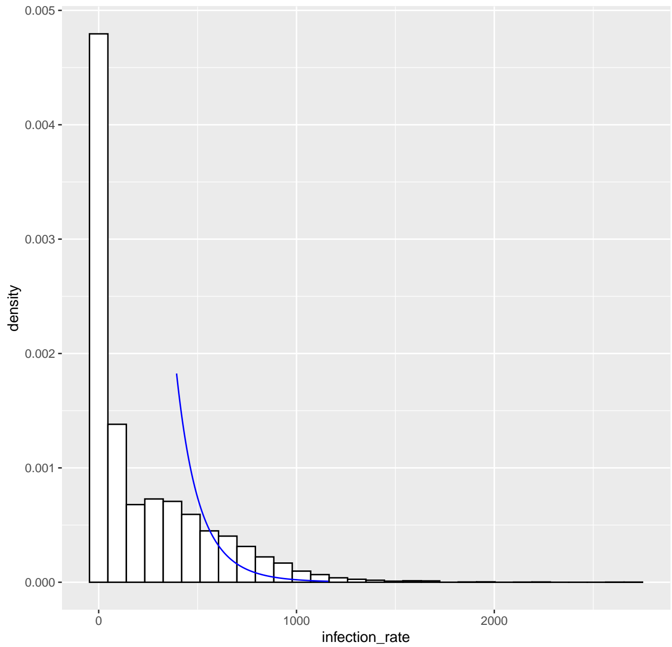
Fitted tail density GPD( 393.8 , 123.48 , 0.09 ), k= 80 -- 23-02-2021
