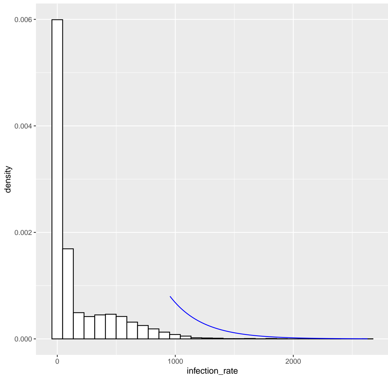
Fitted tail density GPD( 955.3 , 281.58 , 0.01 ), k= 80 -- 22-12-2020
