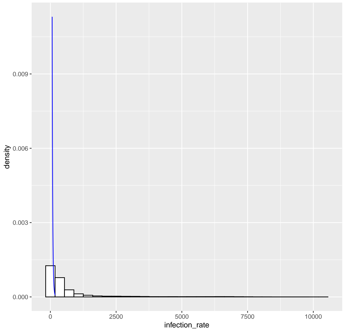
Fitted tail density GPD( 68.3 , 19.93 , 0.09 ), k= 80 -- 22-11-2022
