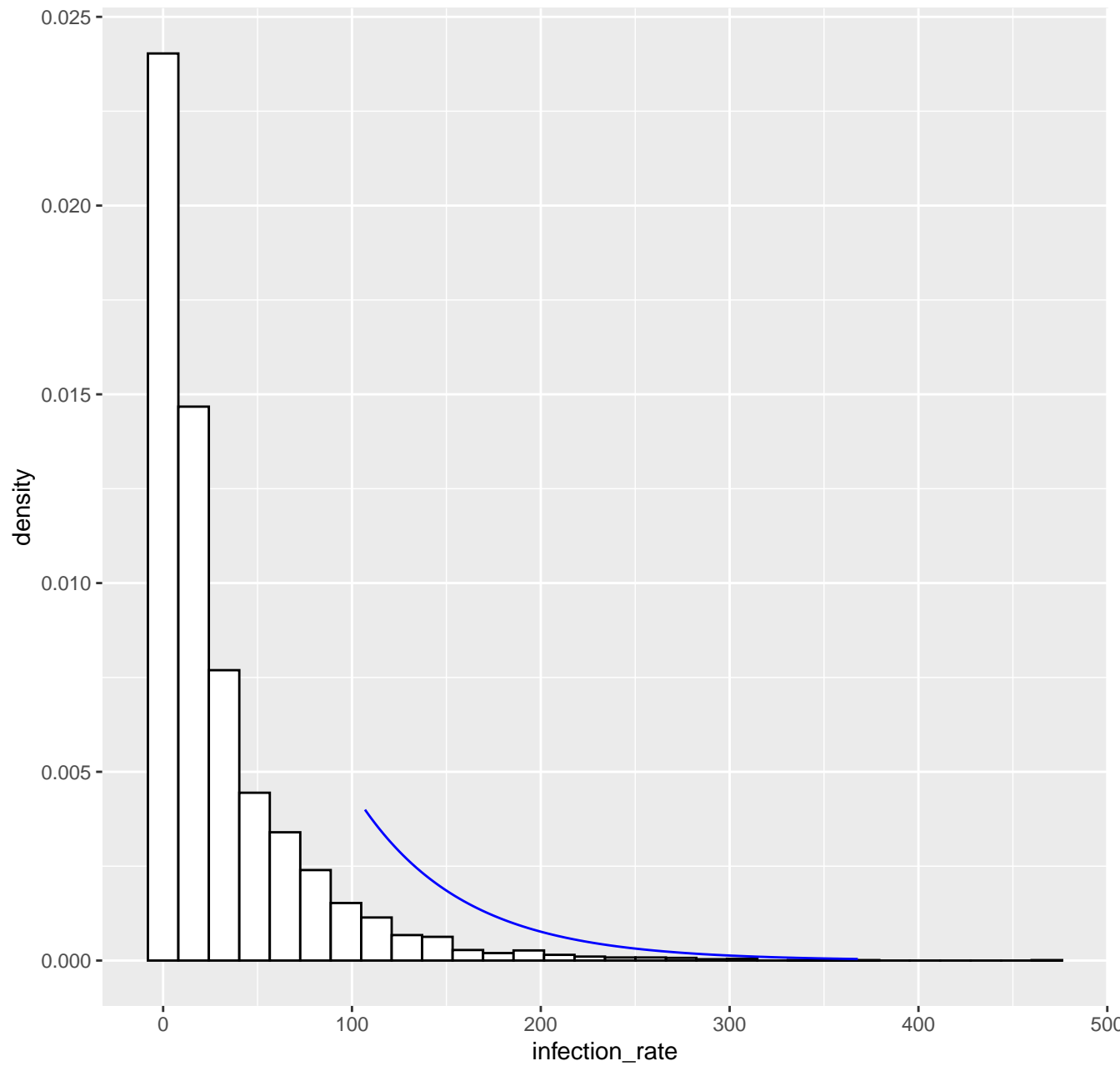
Fitted tail density GPD( 106.9 , 56.37 , 0.01 ), k= 80 -- 22-09-2020
