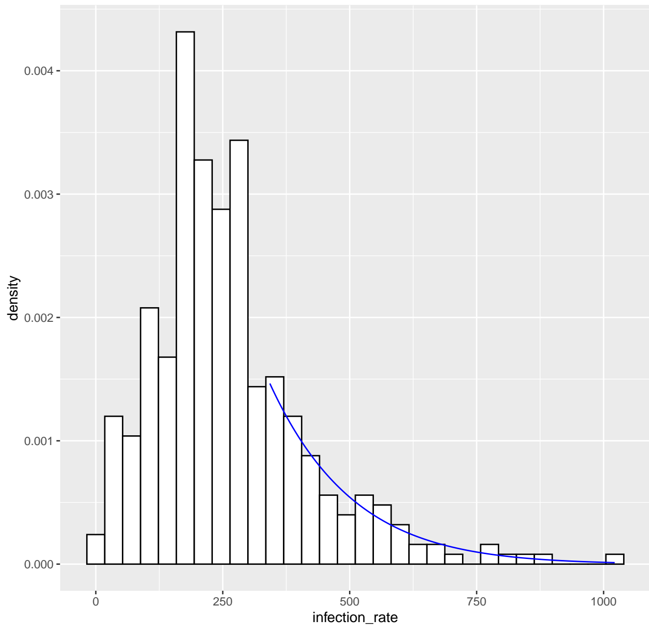
Fitted tail density GPD( 342.8 , 153.89 , -0.06 ), k= 80 -- 22-05-2020
