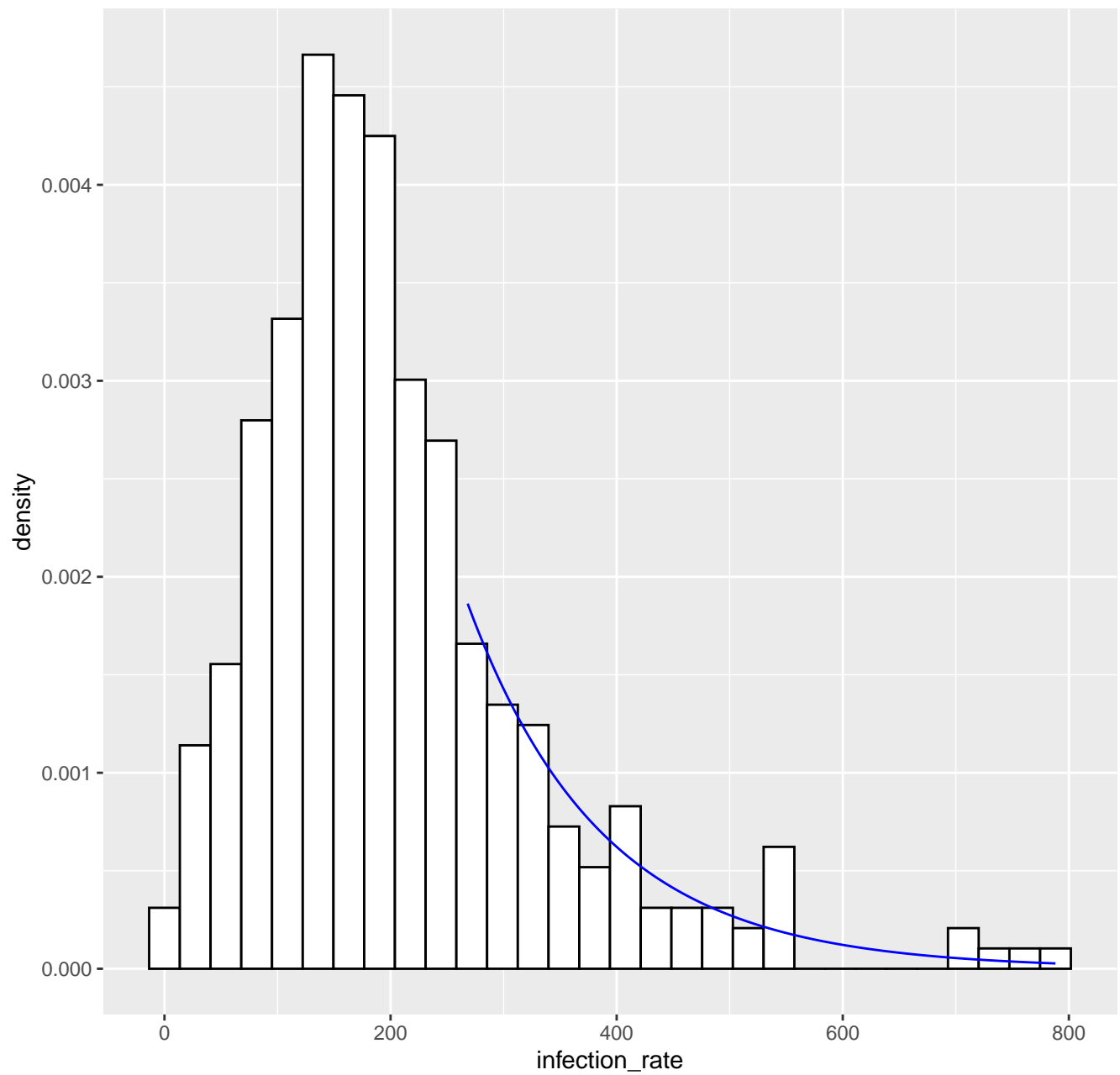
Fitted tail density GPD( 268.2 , 120.96 , 0.02 ), k= 80 -- 22-04-2020
