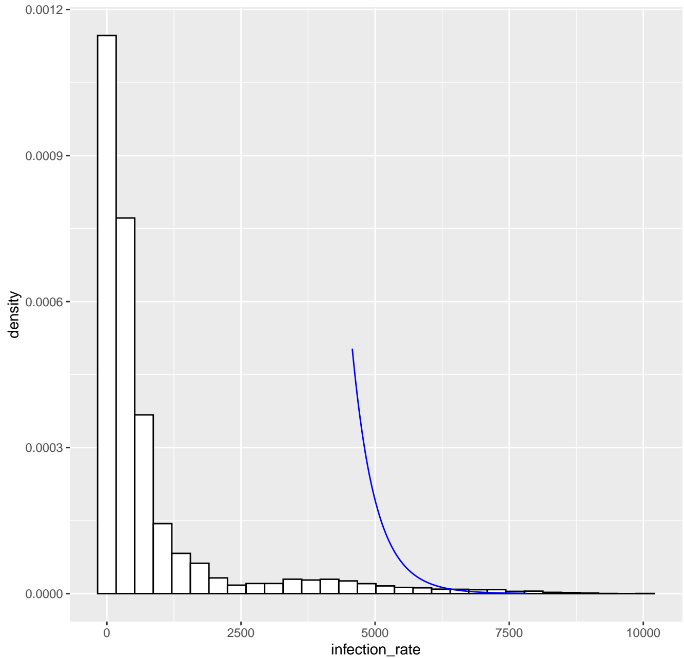
Fitted tail density GPD( 4574.4 , 447.63 , 0.03 ), k= 80 -- 22-03-2022
