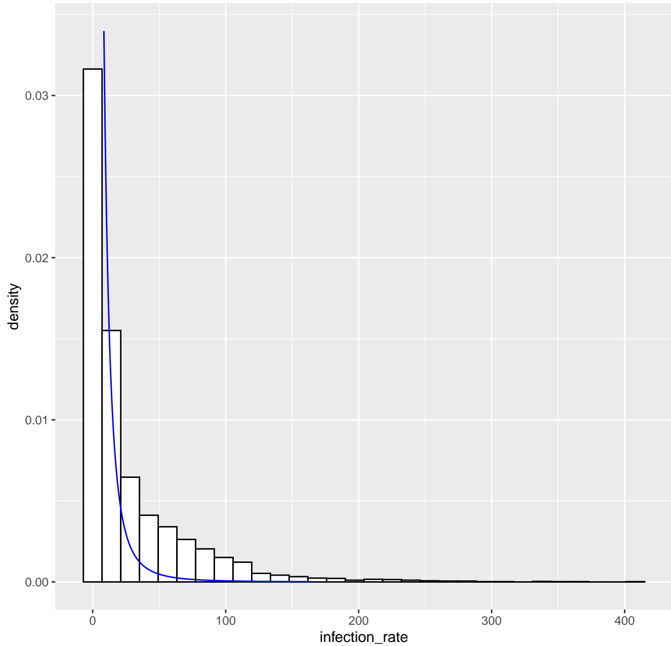
Fitted tail density GPD( 8.4 , 6.63 , 0.5 ), k= 80 -- 21-07-2020
