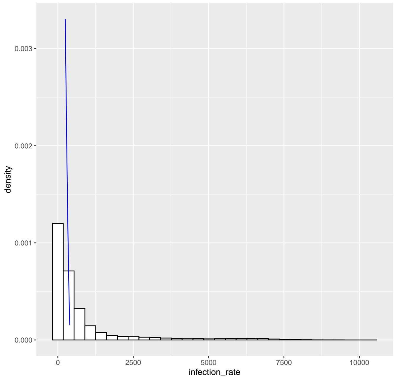
Fitted tail density GPD( 246.4 , 68.17 , -0.4 ), k= 80 -- 21-06-2022
