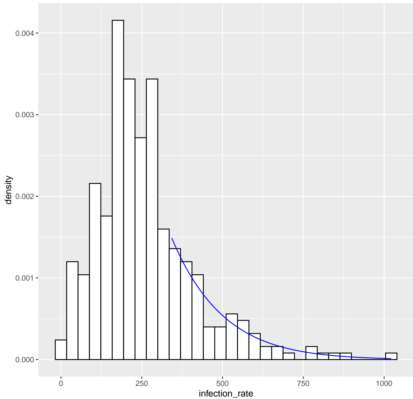
Fitted tail density GPD( 342.8 , 151.35 , -0.05 ), k= 80 -- 21-05-2020
