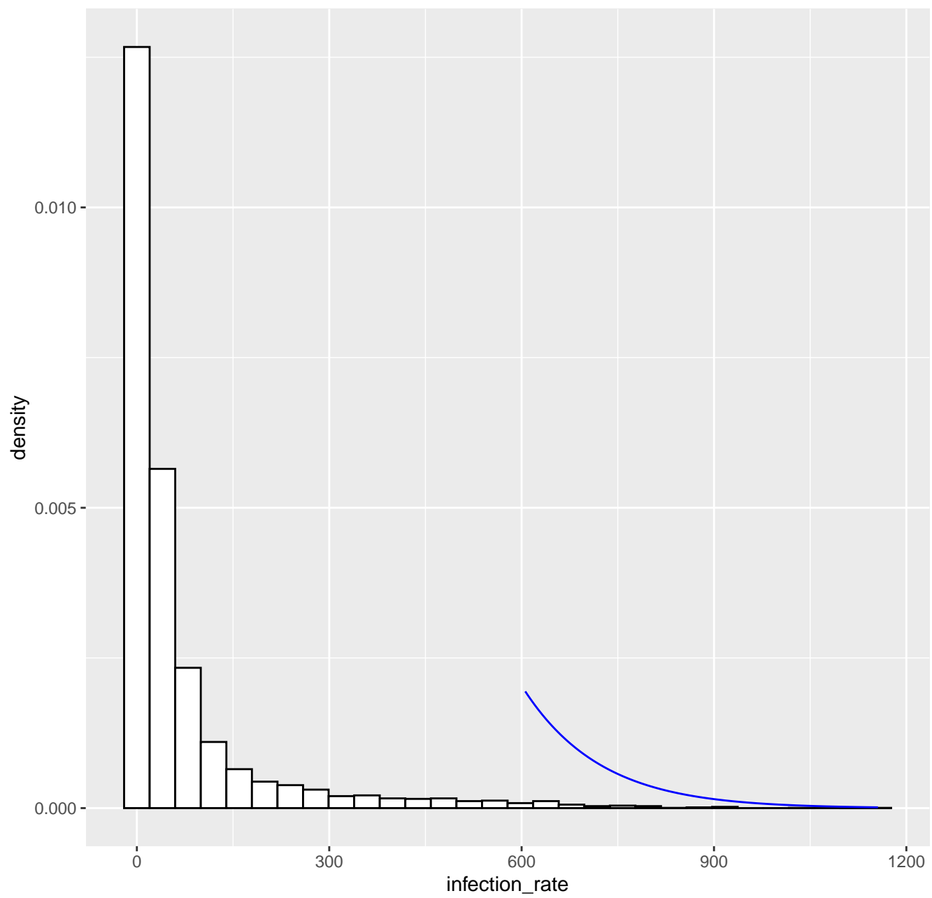
Fitted tail density GPD( 605.7 , 115.96 , -0.03 ), k= 80 -- 20-10-2020
