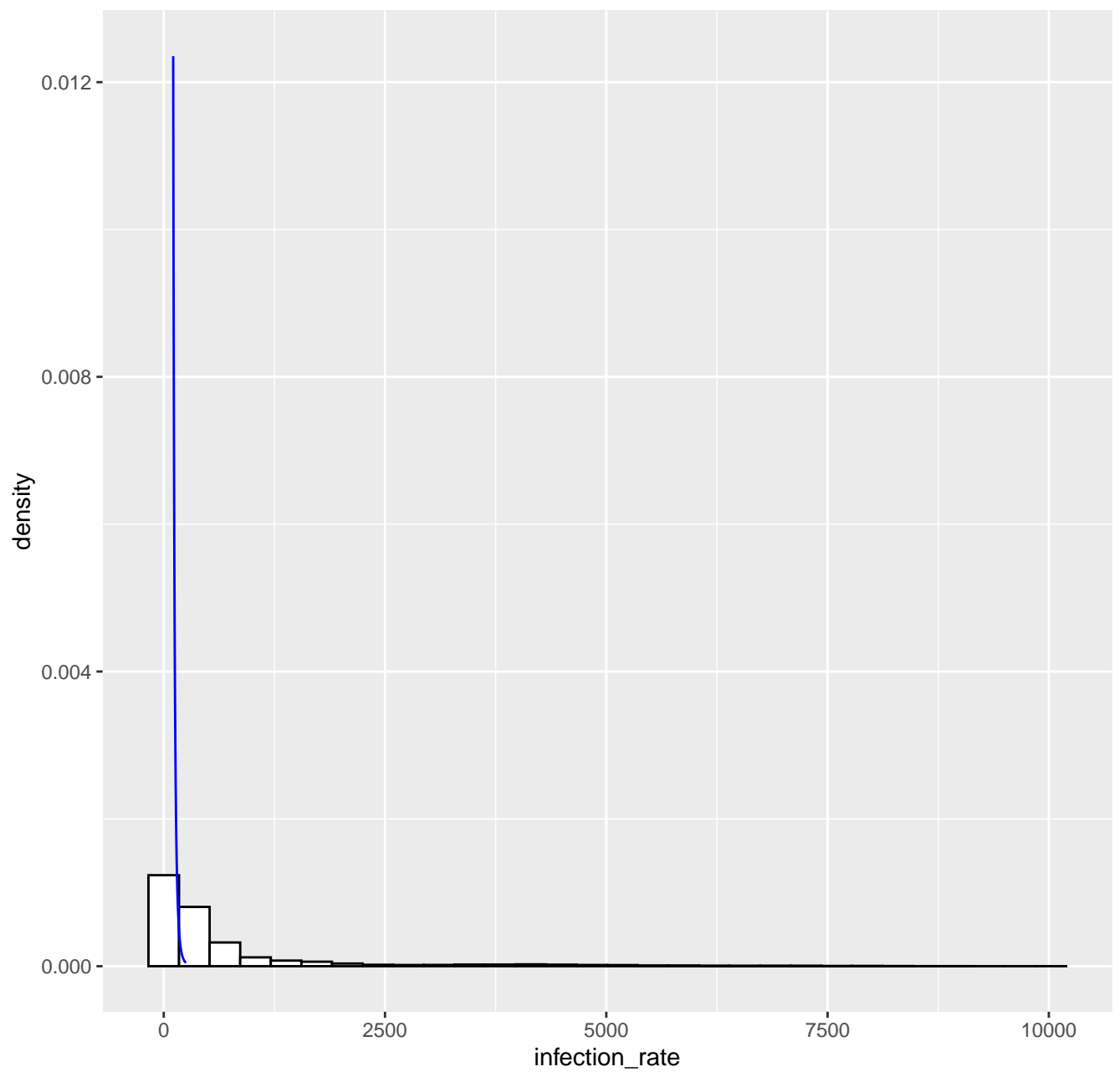
Fitted tail density GPD( 106.9 , 18.24 , 0.22 ), k= 80 -- 20-09-2022
