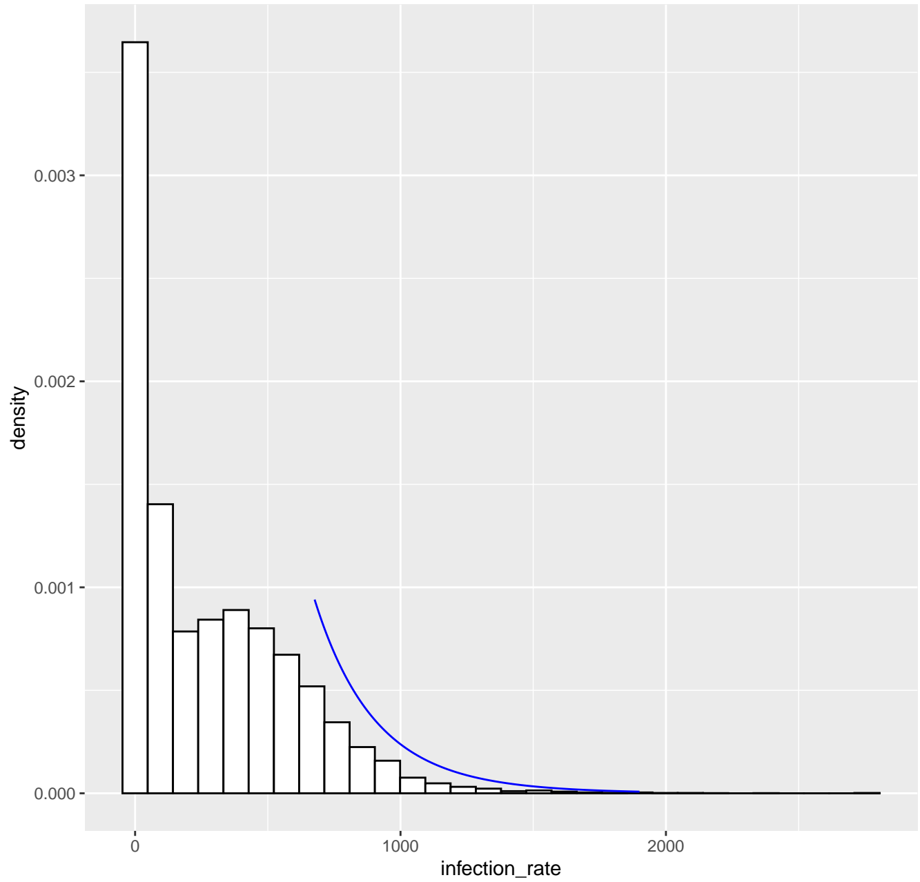
Fitted tail density GPD( 676.4 , 239.61 , 0.05 ), k= 80 -- 20-07-2021
