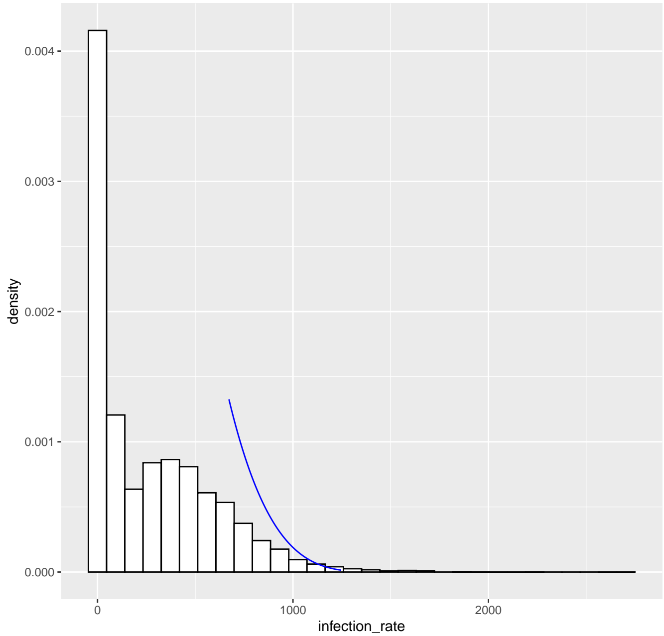
Fitted tail density GPD( 672.4 , 169.93 , -0.2 ), k= 80 -- 20-04-2021
