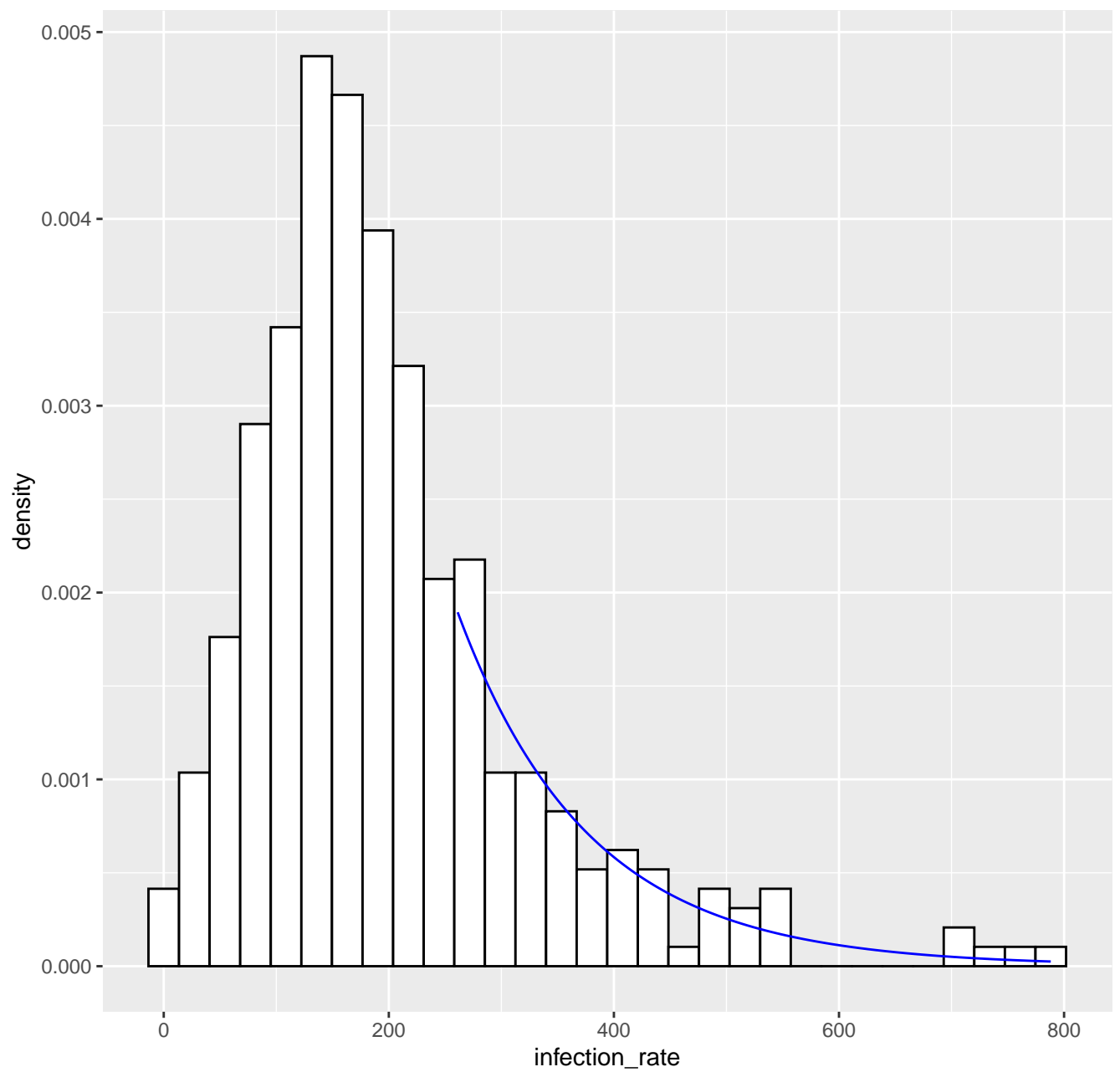
Fitted tail density GPD( 261.2 , 118.95 , 0.02 ), k= 80 -- 20-04-2020
