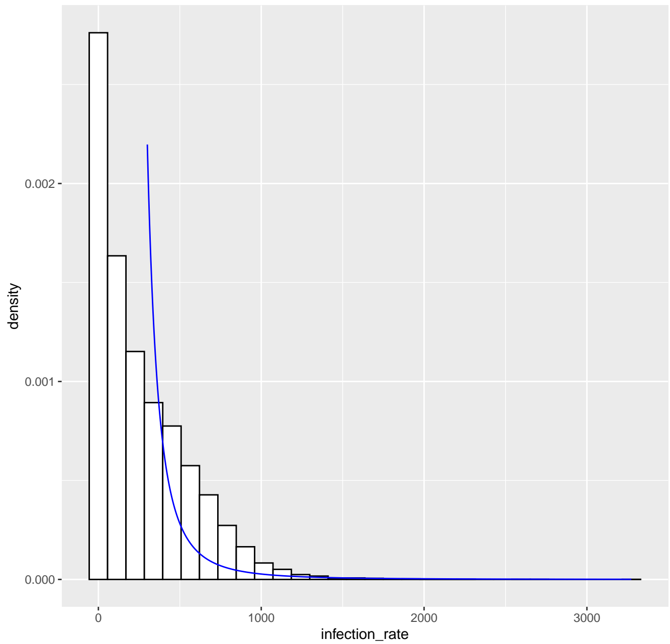
Fitted tail density GPD( 300.5 , 102.57 , 0.55 ), k= 80 -- 19-10-2021
