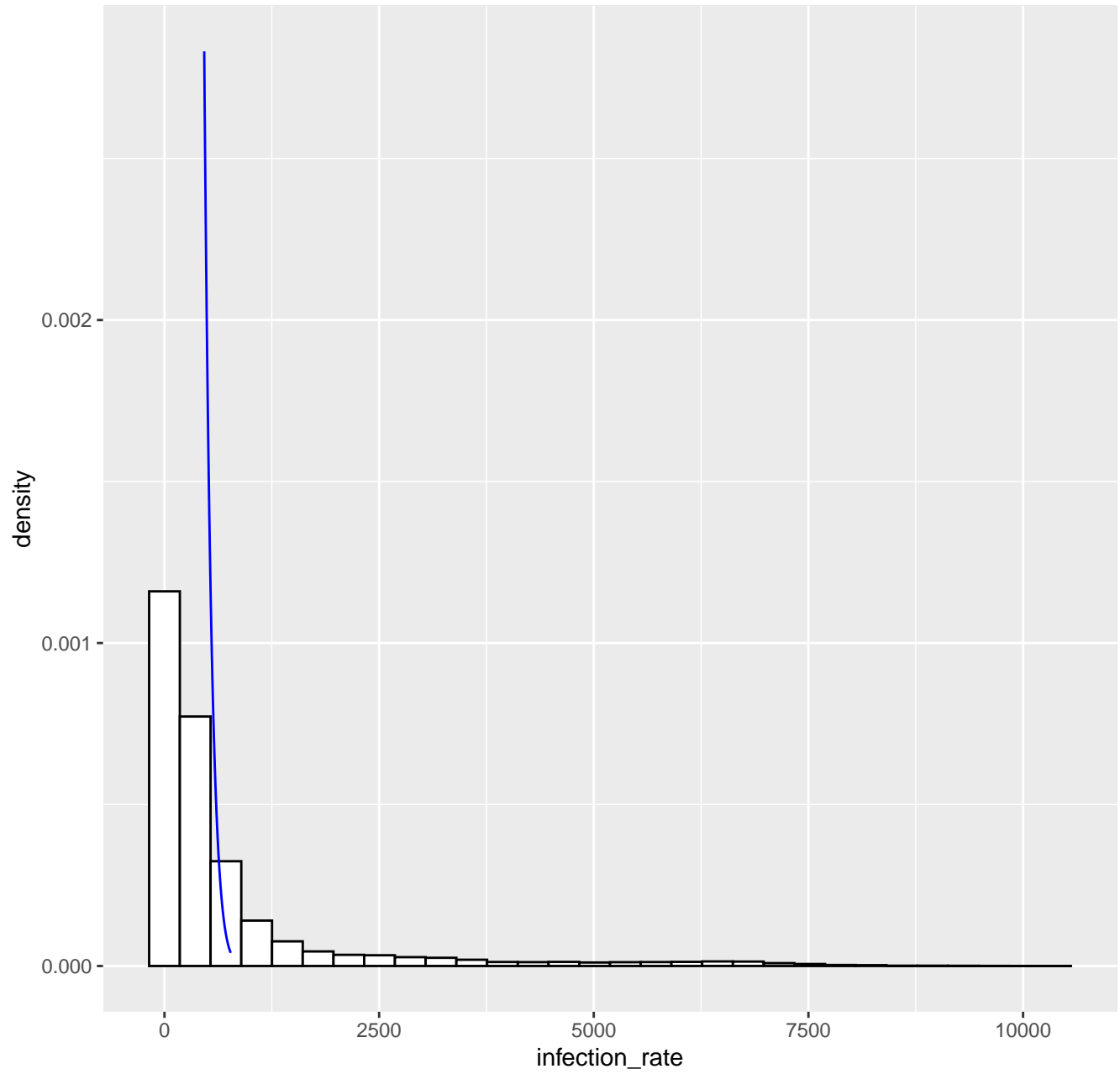
Fitted tail density GPD( 462.9 , 79.58 , -0.08 ), k= 80 --- 19-07-2022
