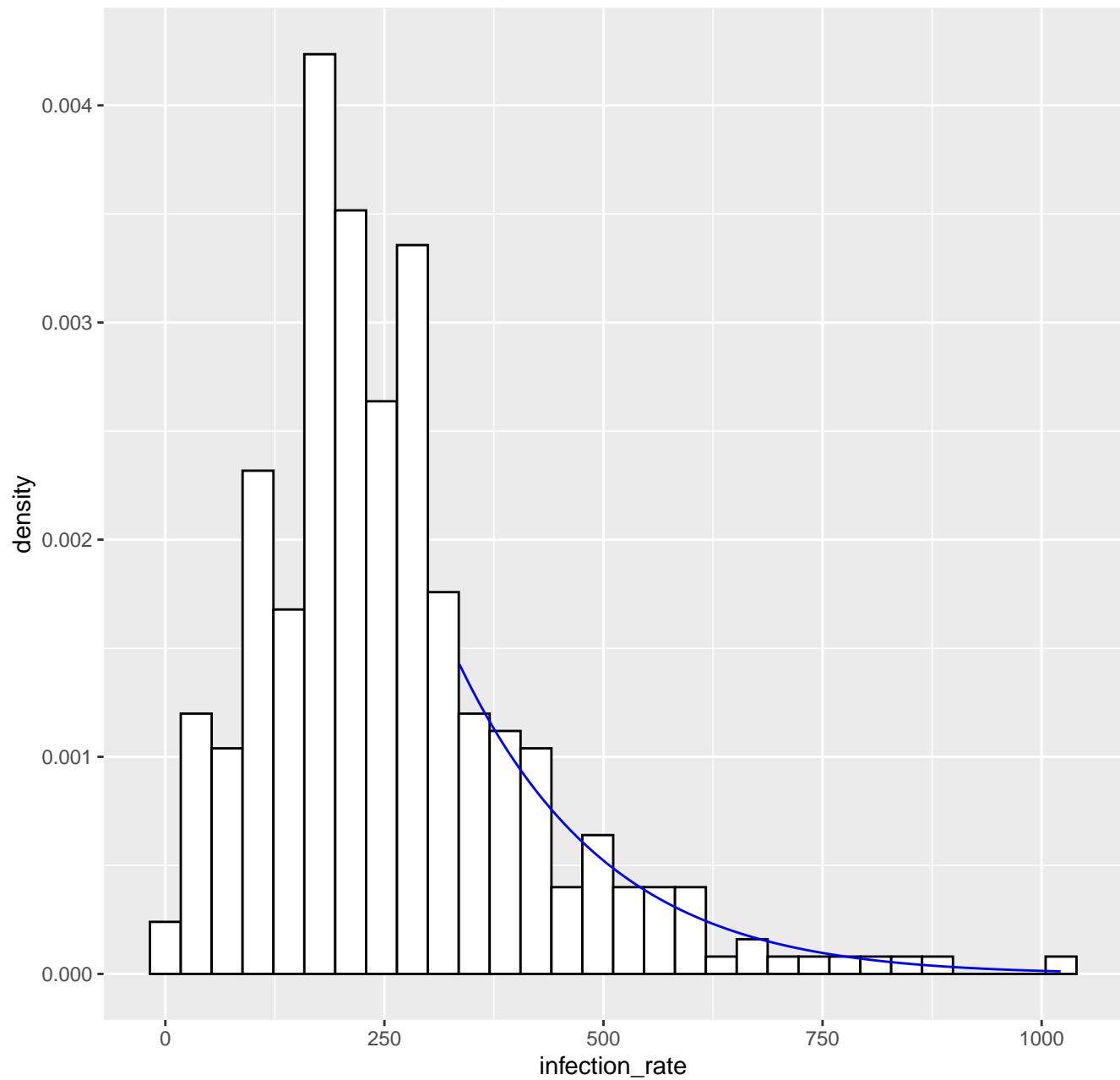
Fitted tail density GPD( 335.7 , 158.04 , -0.07 ), k= 80 -- 19-05-2020
