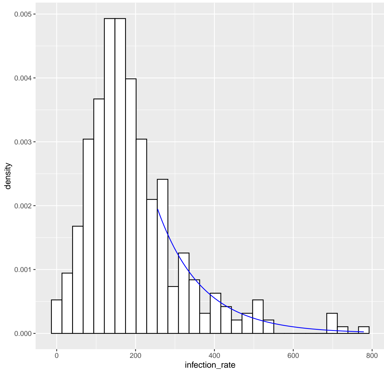
Fitted tail density GPD( 255.9 , 115.71 , 0.03 ), k= 80 -- 19-04-2020
