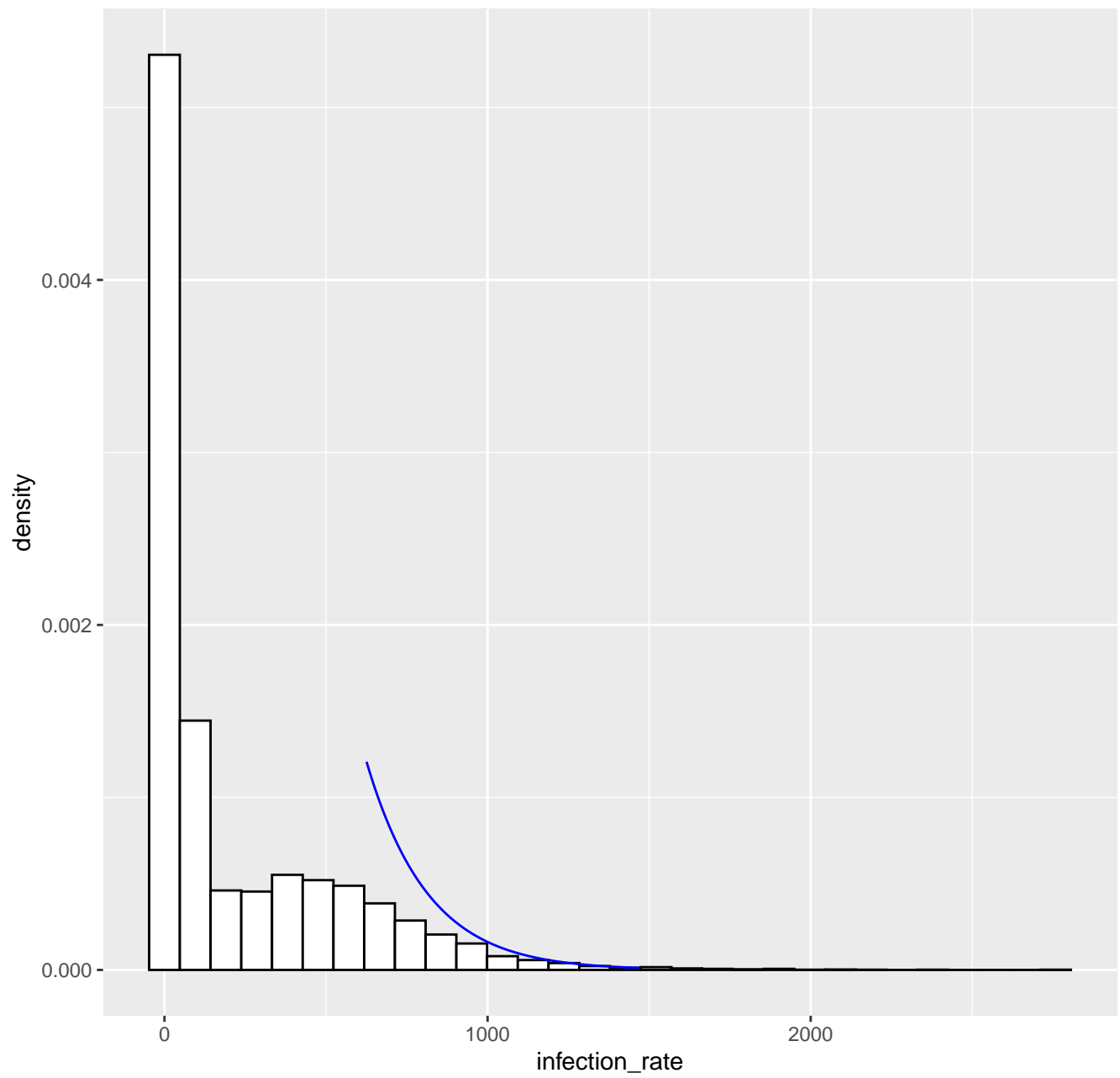
Fitted tail density GPD( 625.4 , 186.71 , -0.02 ), k= 80 -- 19-01-2021
