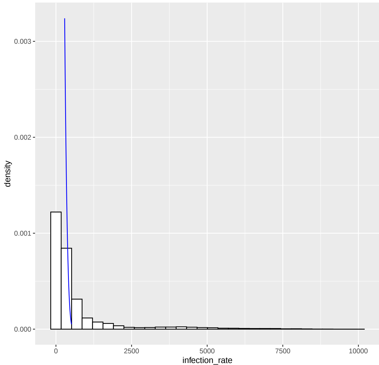
Fitted tail density GPD( 287.5 , 69.55 , -0.2 ), k= 80 -- 18-10-2022
