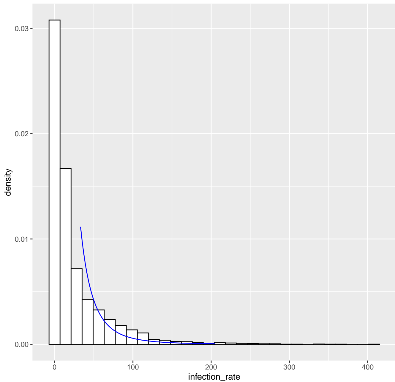
Fitted tail density GPD( 33.2 , 20.19 , 0.32 ), k= 80 -- 18-08-2020
