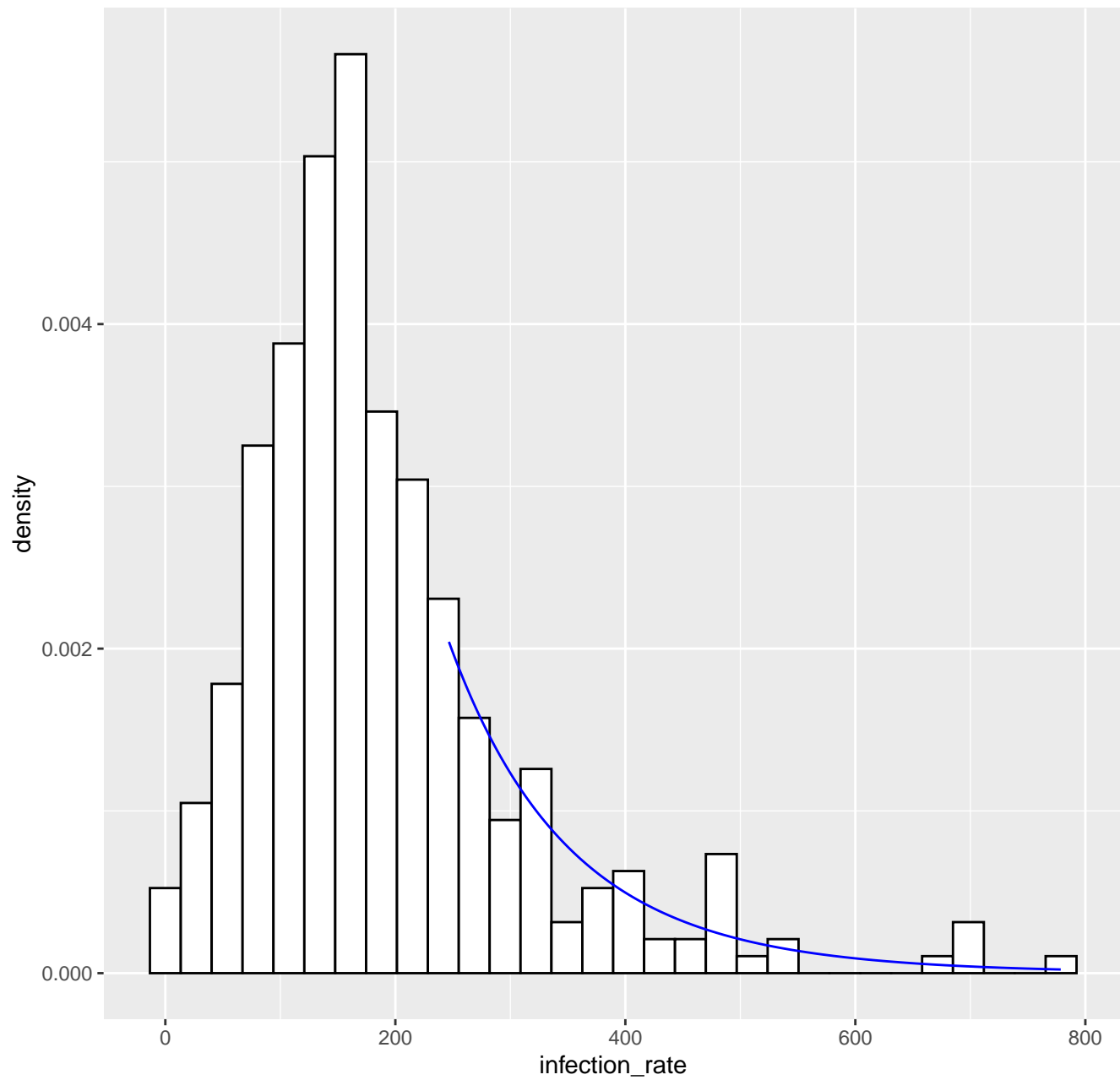
Fitted tail density GPD( 246.6 , 110.37 , 0.06 ), k= 80 -- 18-04-2020
