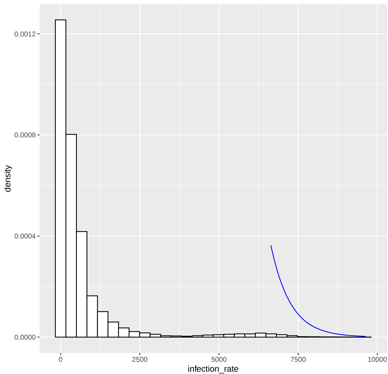
Fitted tail density GPD( 6638.7 , 620.78 , 0 ), k= 80 -- 18-02-2022
