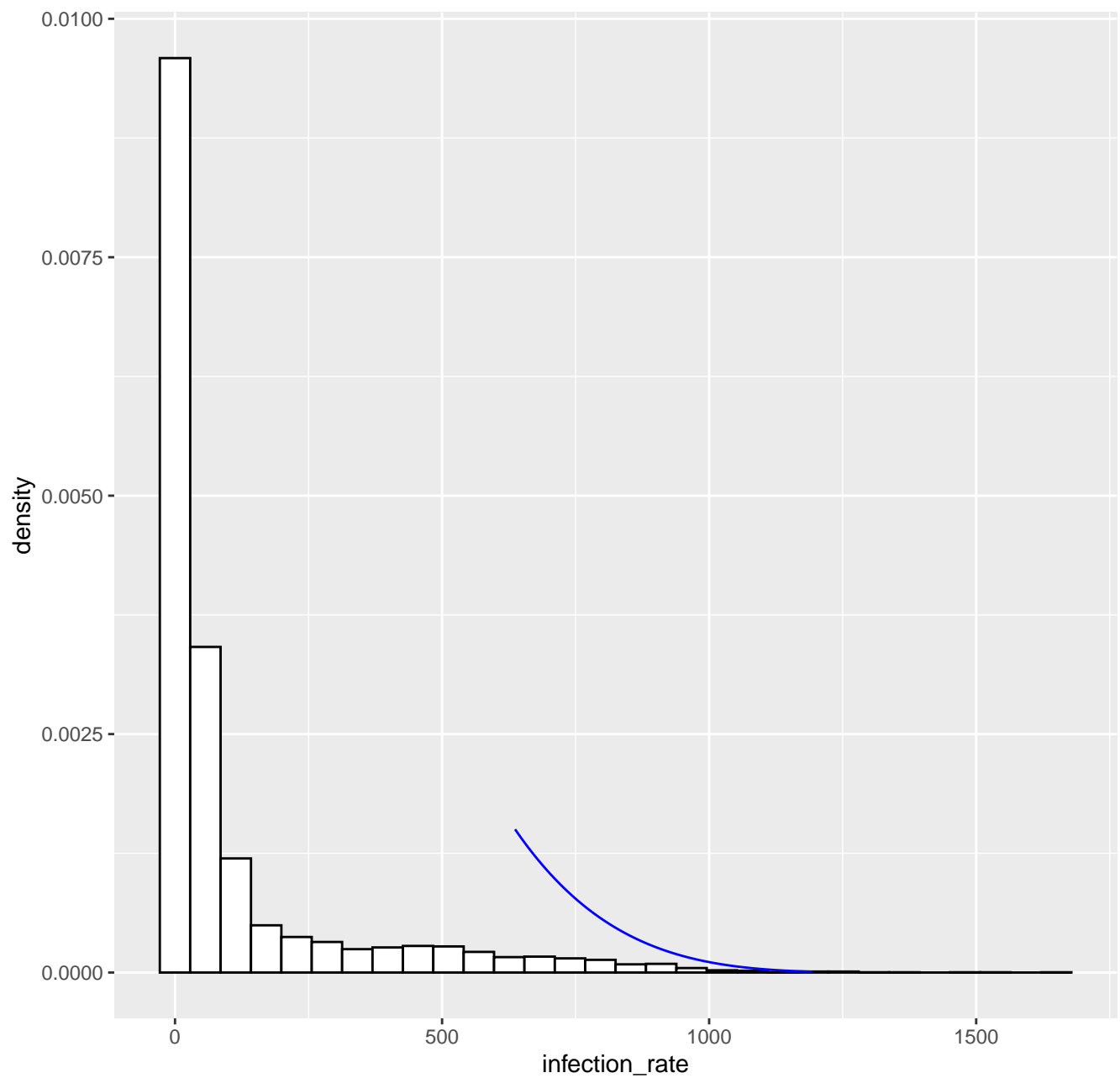
Fitted tail density GPD( 636.7 , 150.04 , -0.19 ), k= 80 --- 17-11-2020
