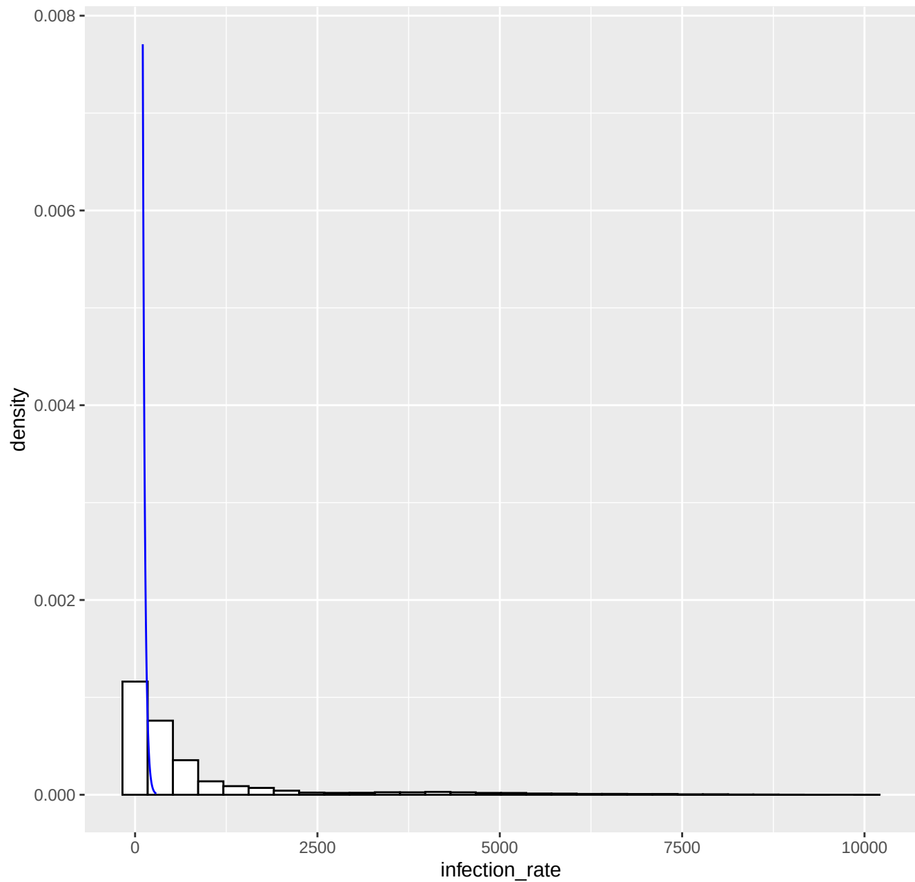
Fitted tail density GPD( 105.3 , 29.24 , -0.01 ), k= 80 -- 17-05-2022
