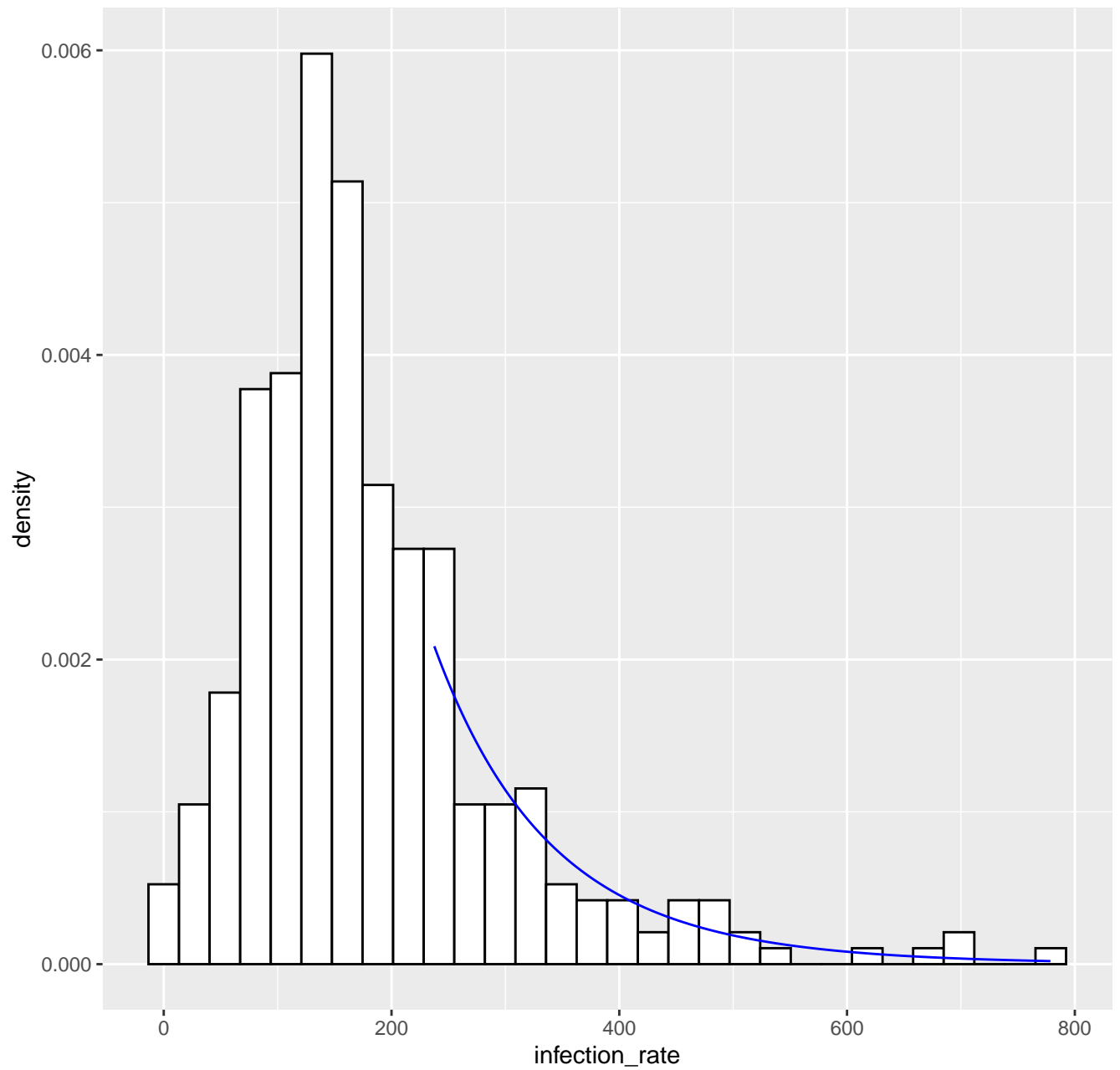
Fitted tail density GPD( 237.6 , 107.97 , 0.06 ), k= 80 --- 17-04-2020
