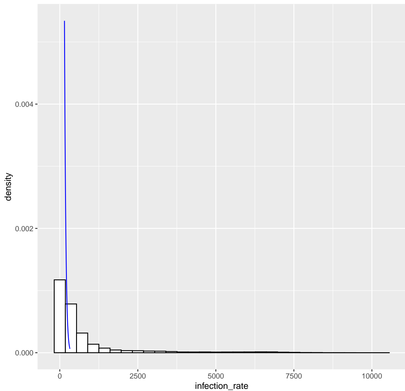
Fitted tail density GPD( 150.1 , 42.2 , -0.05 ), k= 80 -- 16-08-2022
