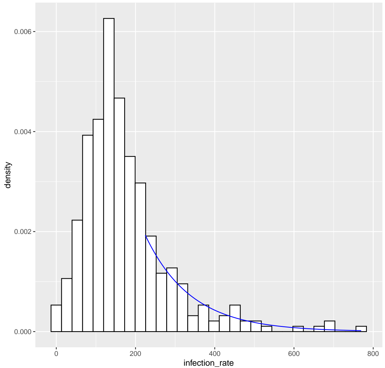
Fitted tail density GPD( 224.6 , 116.79 , 0.01 ), k= 80 --- 16-04-2020
