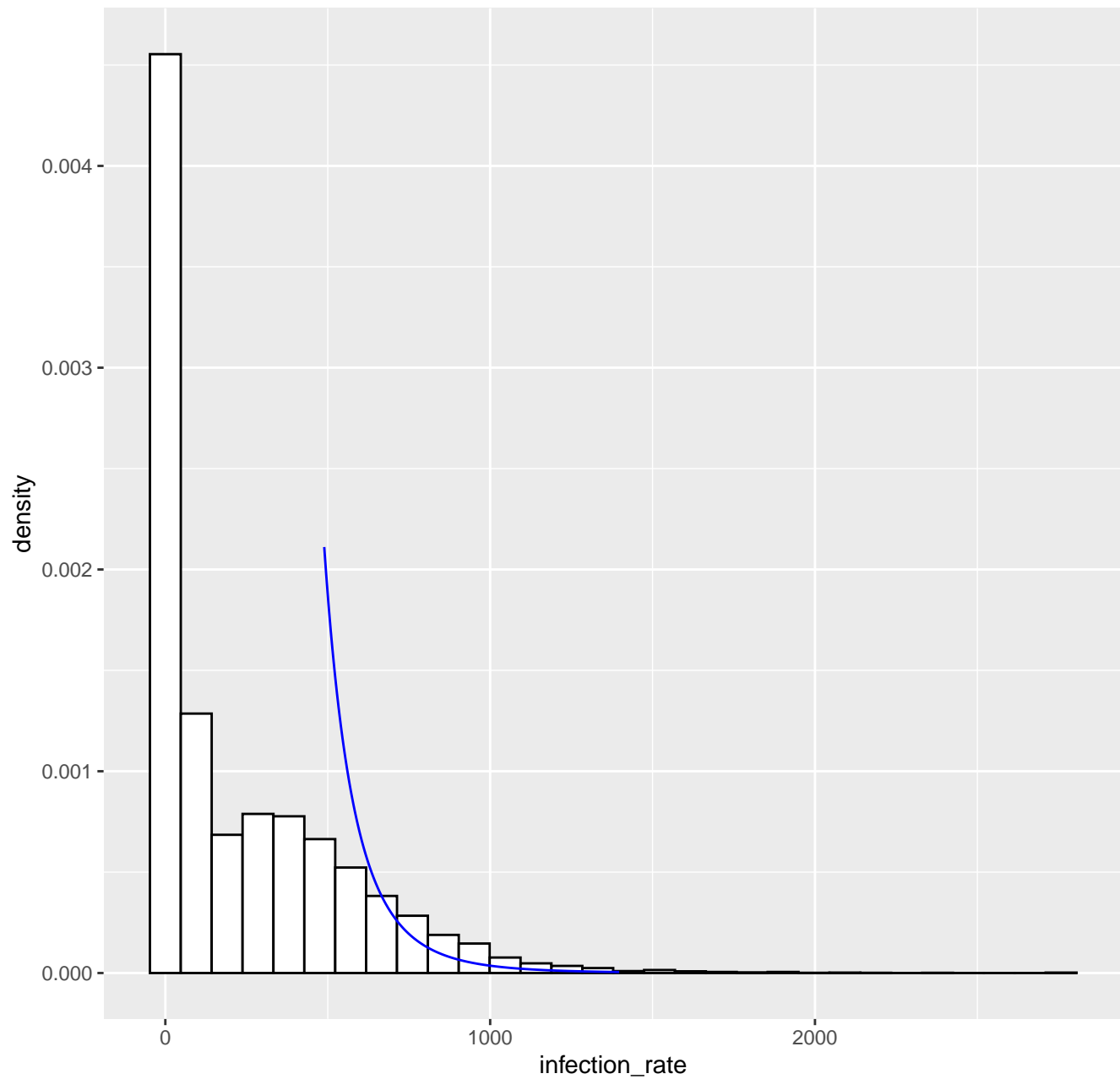
Fitted tail density GPD( 489.2 , 106.74 , 0.19 ), k= 80 -- 16-03-2021
