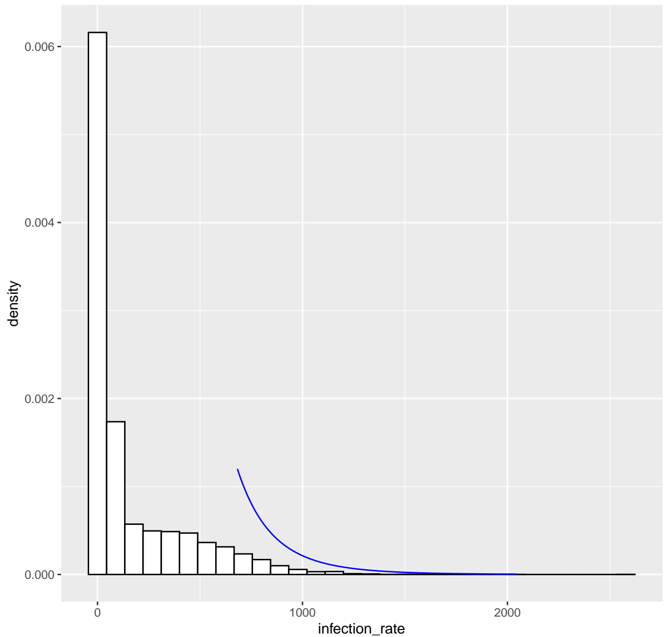
Fitted tail density GPD( 682.5 , 187.83 , 0.13 ), k= 80 --- 15-12-2020
