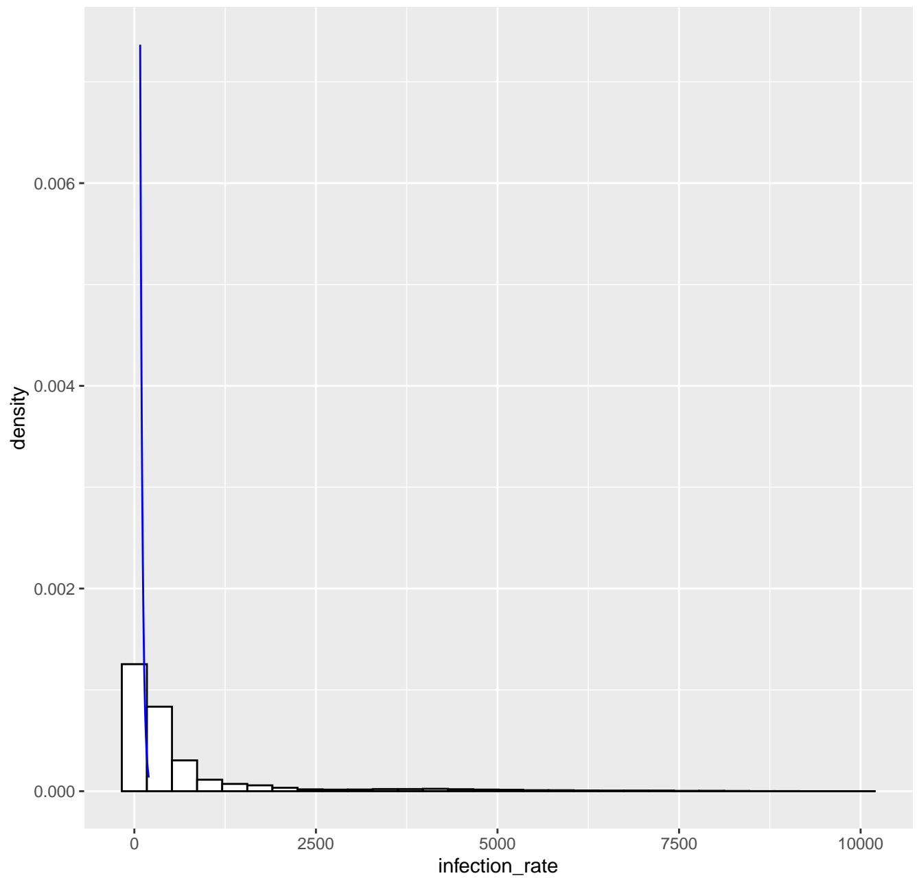
Fitted tail density GPD( 80.1 , 30.59 , -0.03 ), k= 80 -- 15-11-2022
