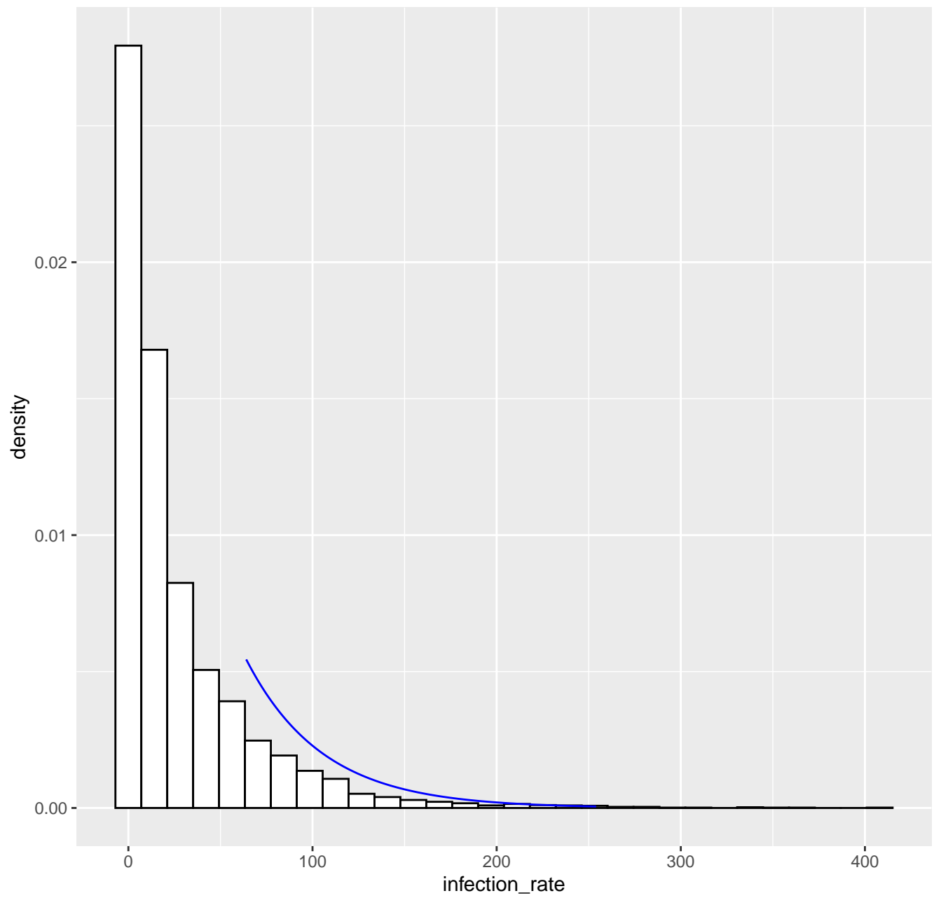
Fitted tail density GPD( 64 , 41.39 , 0 ), k= 80 -- 15-09-2020
