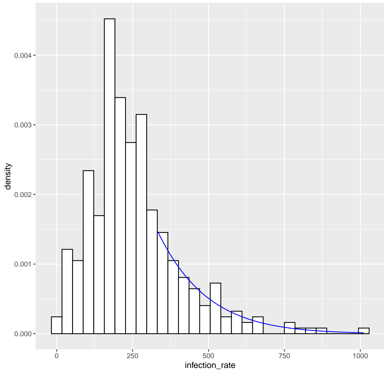
Fitted tail density GPD( 333.1 , 153.71 , -0.05 ), k= 80 -- 15-05-2020
