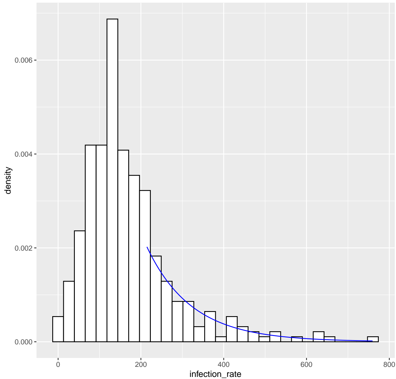
Fitted tail density GPD( 214.5 , 111.46 , 0.03 ), k= 80 --- 15-04-2020
