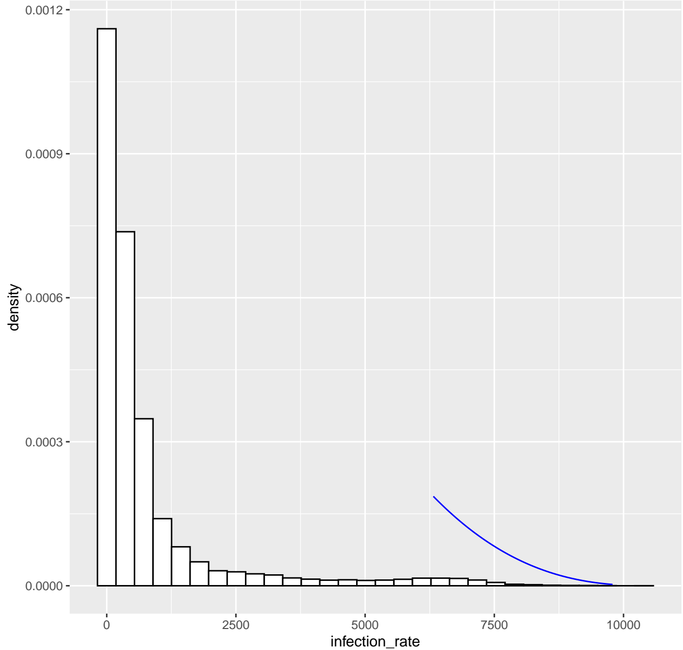
Fitted tail density GPD( 6320.6 , 1210.21 , -0.28 ), k= 80 -- 15-03-2022
