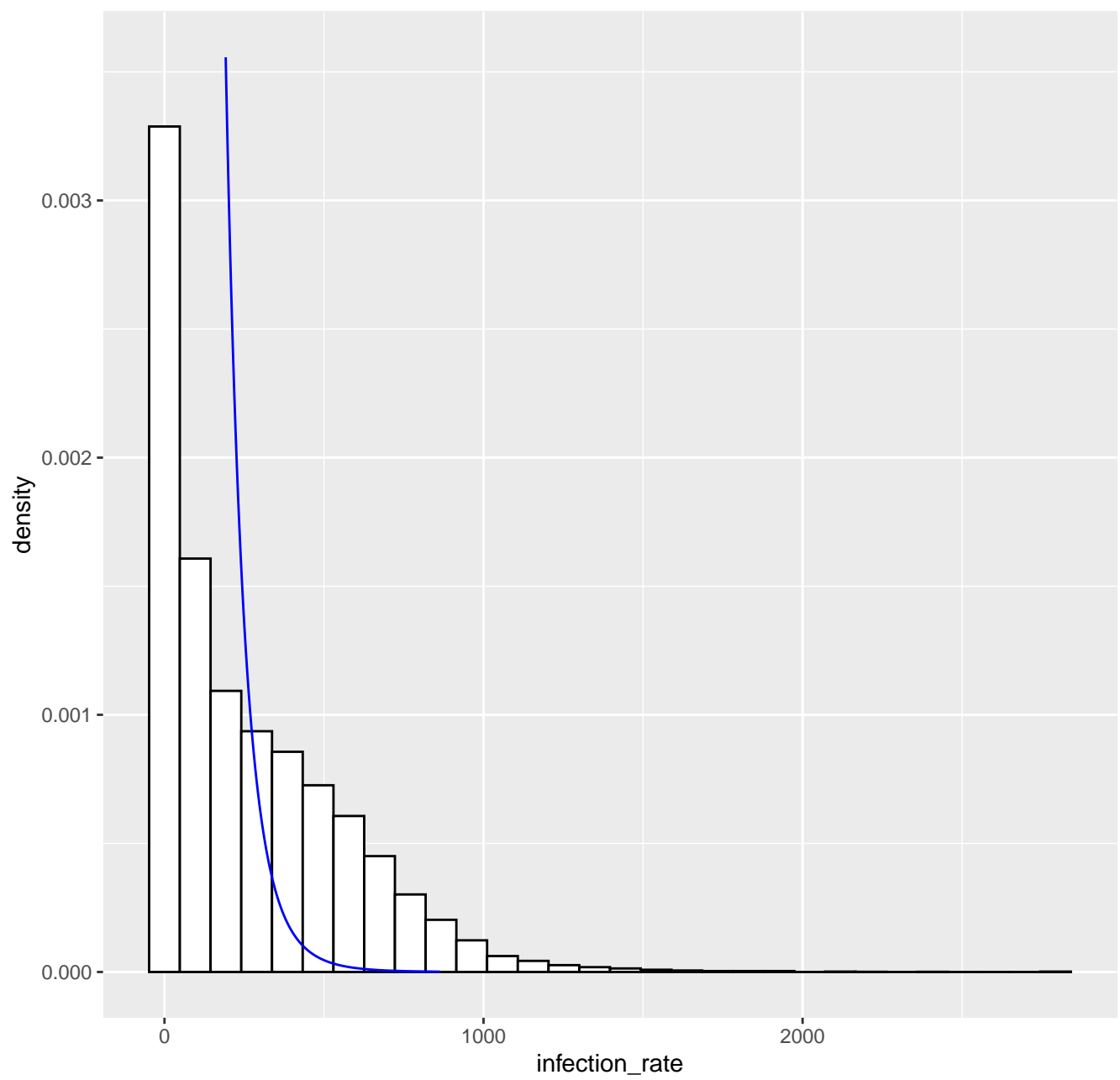
Fitted tail density GPD( 191.9 , 63.36 , 0.1 ), k= 80 -- 14-09-2021
