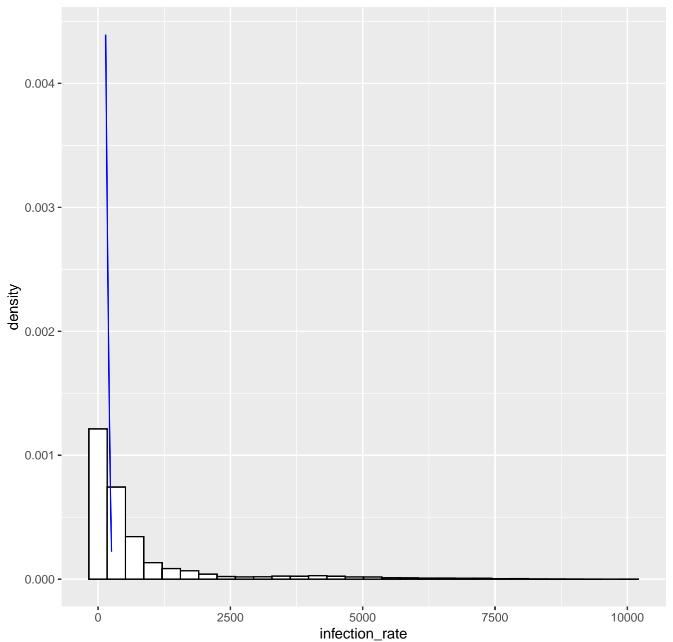
Fitted tail density GPD( 144.6 , 51.3 , -0.4 ), k= 80 -- 14-06-2022
